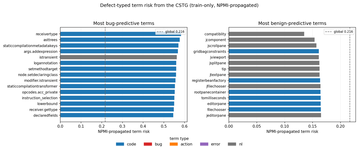
Figure 9: Defect-typed, NPMI-propagated term risk (train-only). The bug-predictive terms localise the known fault-prone Groovy subsystems.
