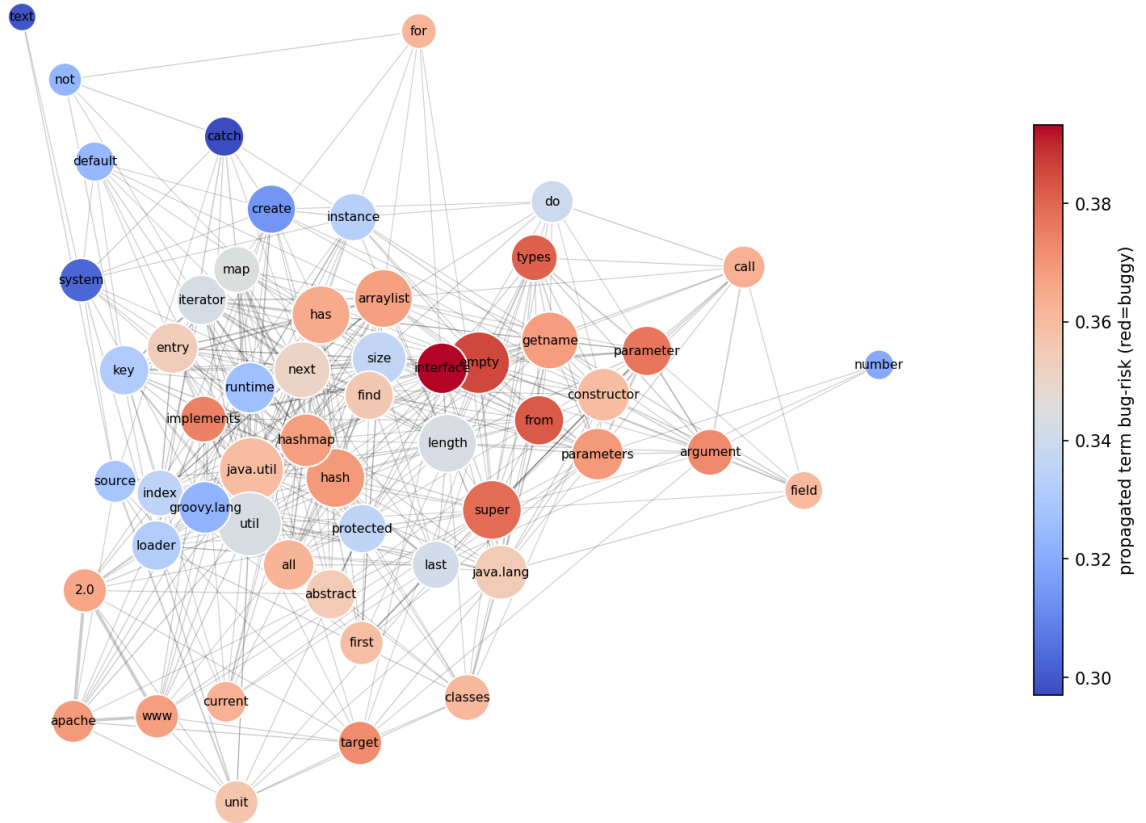
CSTG term co-occurrence graph: NPMI hubs, node colour = propagated bug-risk (semantic communities emerge: buggy type-system/generics terms in red, benign control-flow/instantiation terms in blue)
